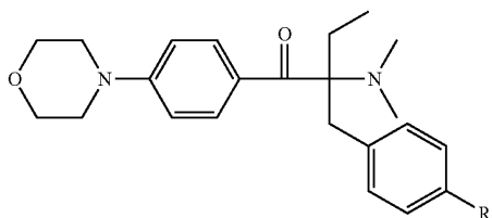
Chemical Formula 11
