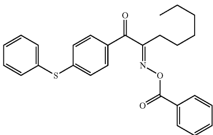
Chemical Formula 13
