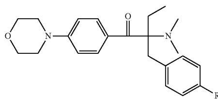
Chemical Formula 10
