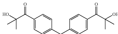
Chemical Formula 5
