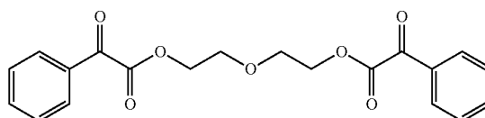
Chemical Formula 6
