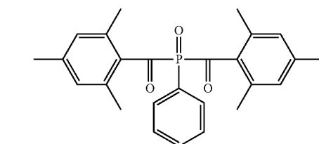
Chemical Formula 7
