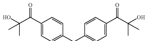
Chemical Formula 5
