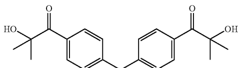
Chemical Formula 5
