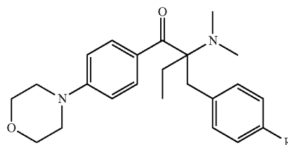
Chemical Formula 9
