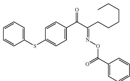
Chemical Formula 13
