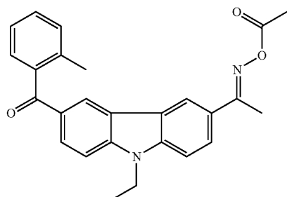
Chemical Formula 14
