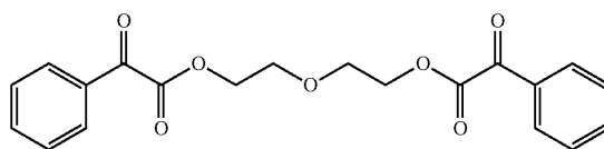
Chemical Formula 6
