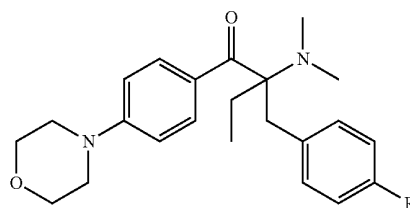
Chemical Formula 10
