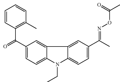
Chemical Formula 14
