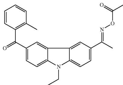
Chemical Formula 14
