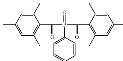
Chemical Formula 7
