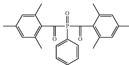
Chemical Formula 7
