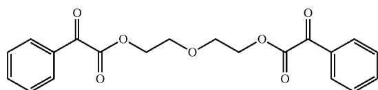
Chemical Formula 5
