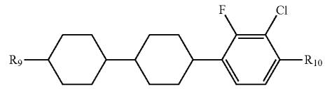
Chemical Formula 20
