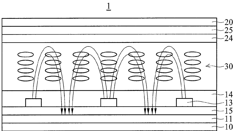
FIG. 1 (RELATED ART)
