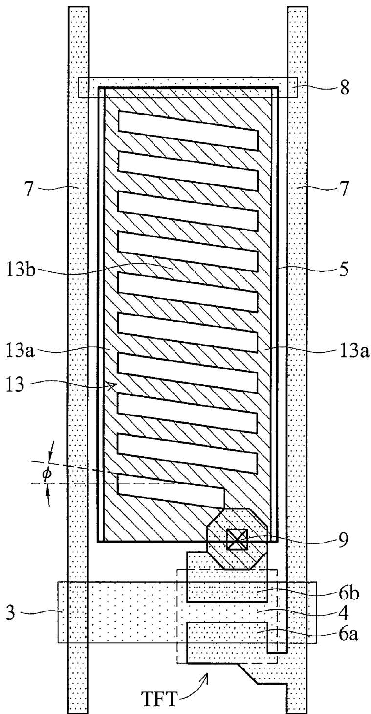
FIG. 2 (RELATED ART)
