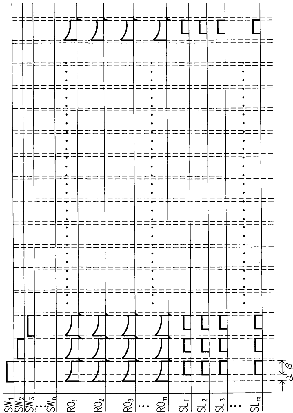
Fig. 5(PRIOR ART)
