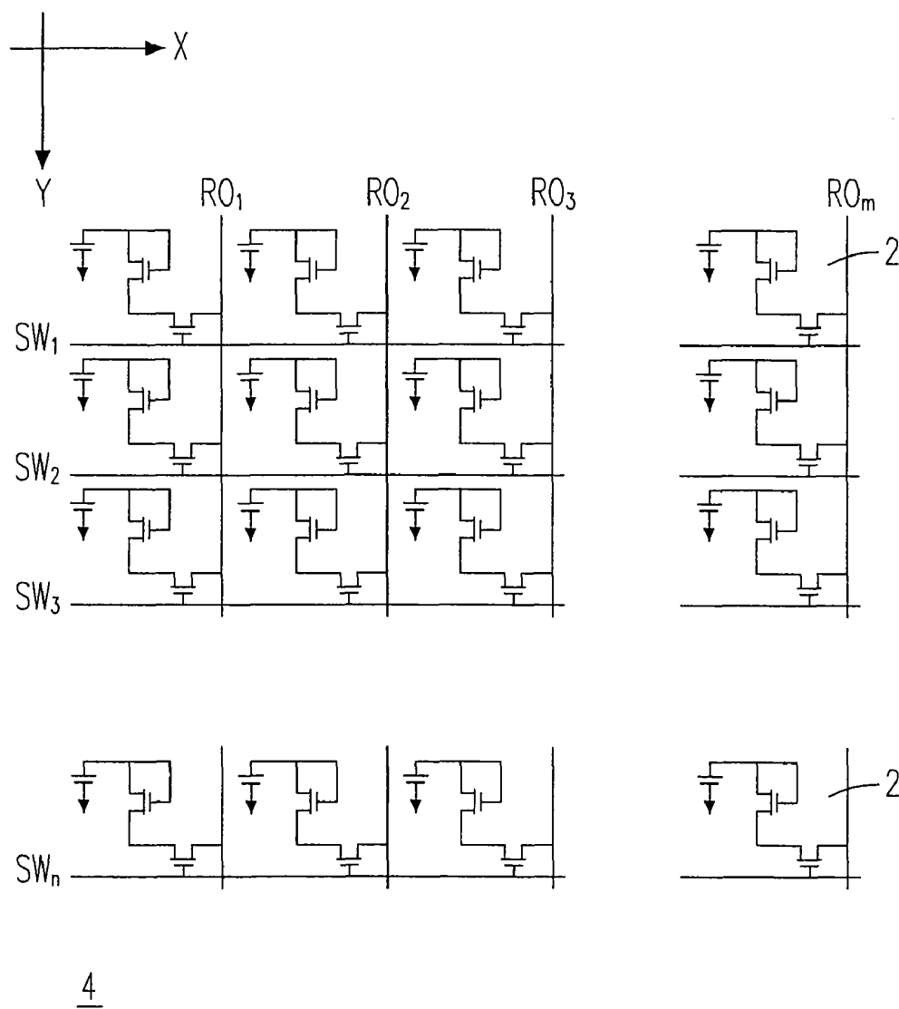
Fig. 4 (PRIOR ART)
