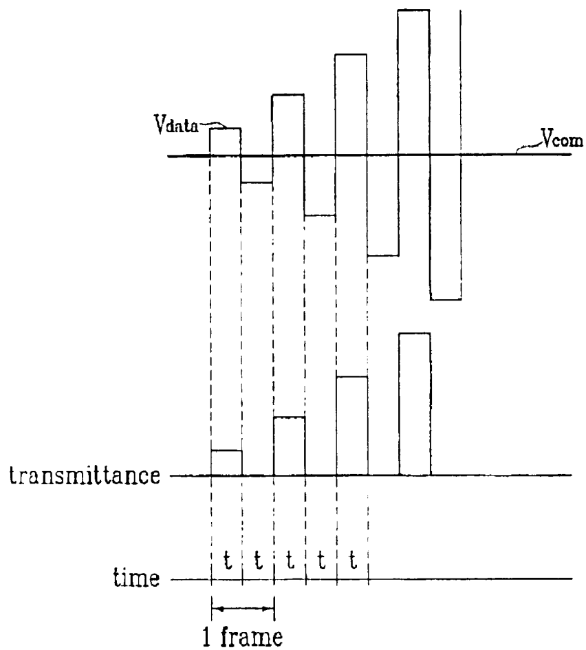
FIG. 4 Related Art
