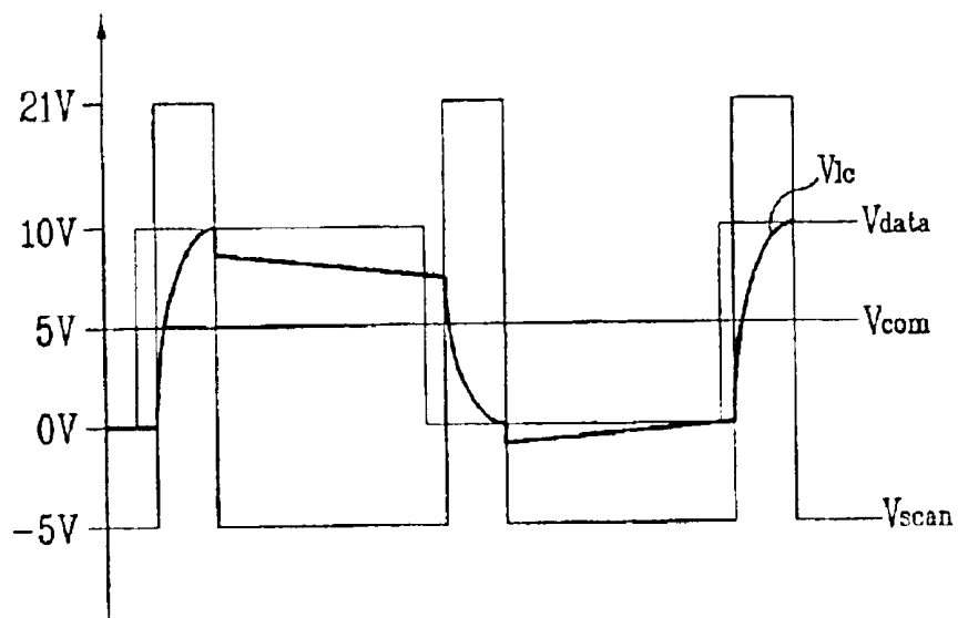
FIG. 2 Related Art
