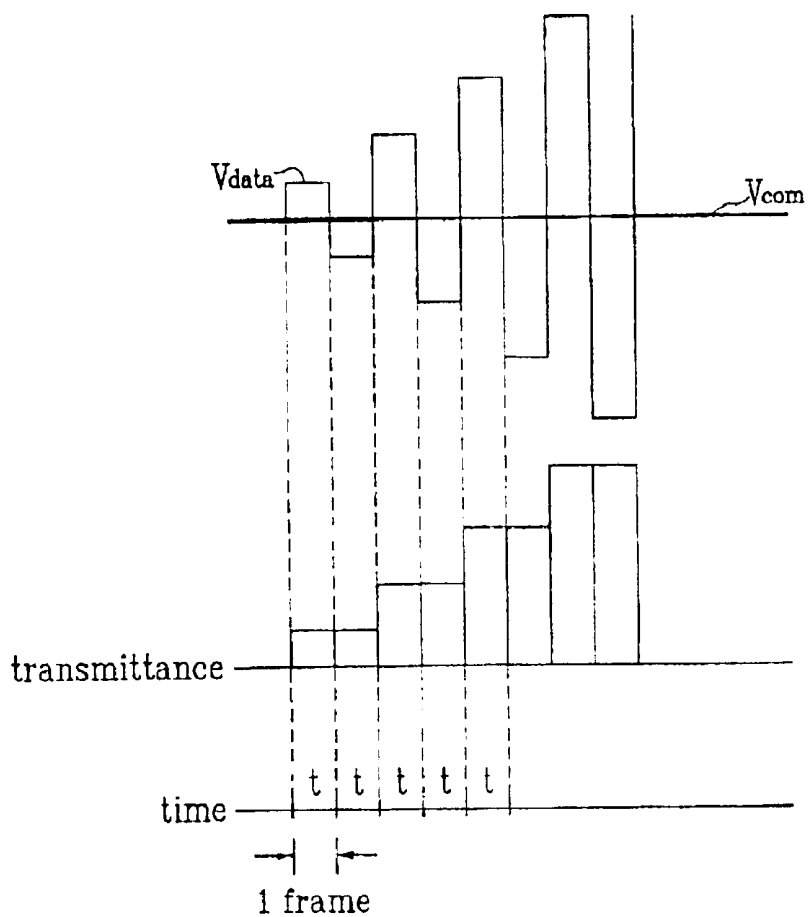
FIG. 2 Related Art
