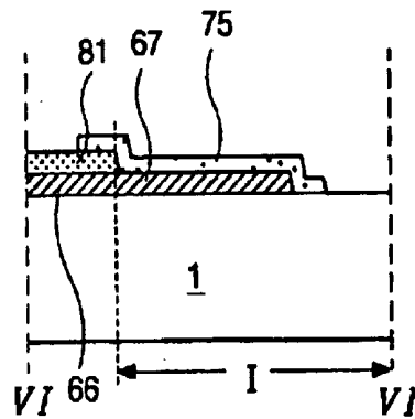
FIG. 6C (RELATED ART)
