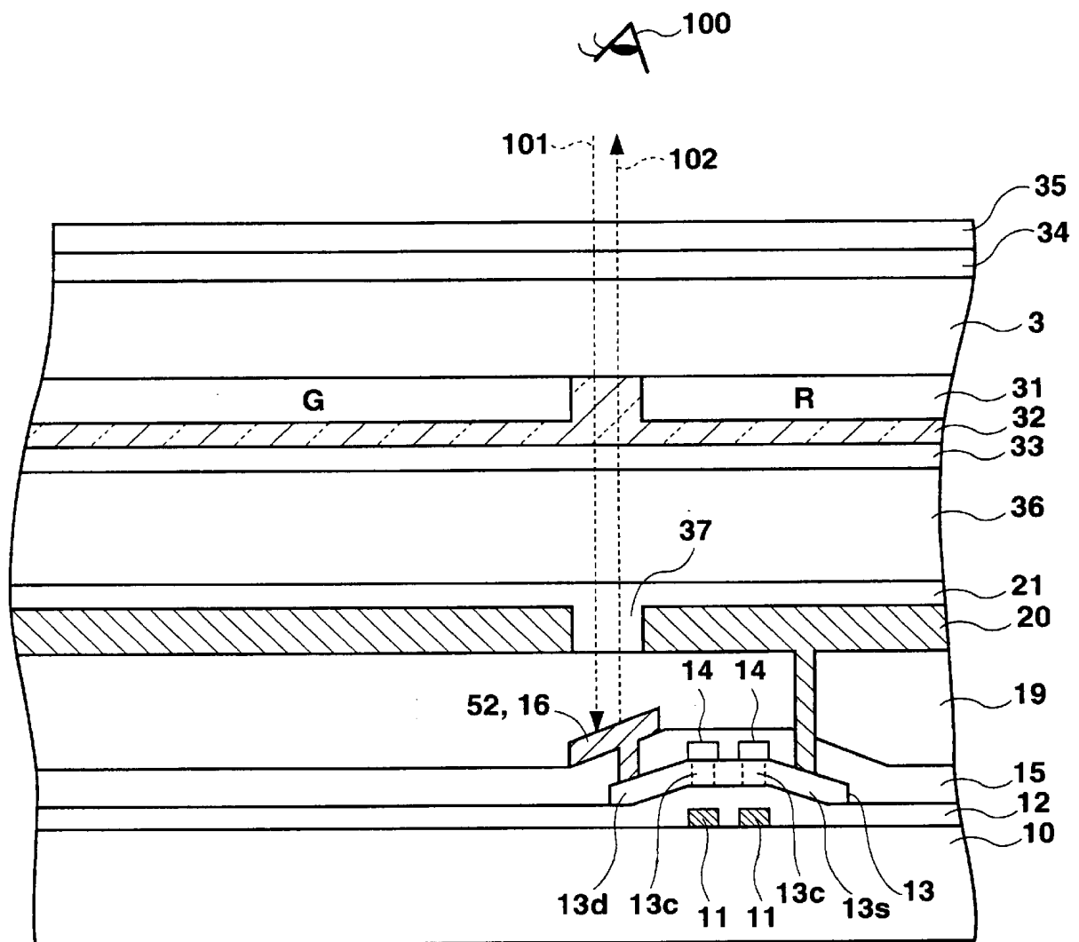
Fig. 2 PRIOR ART
