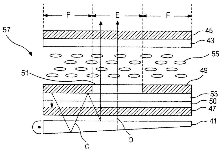
Fig. 3 (Related Art)
