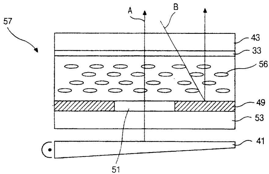
Fig.2 (Related Art)
