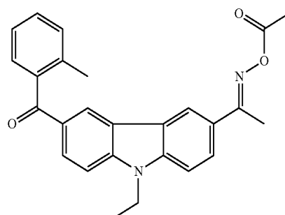
Chemical Formula 14
