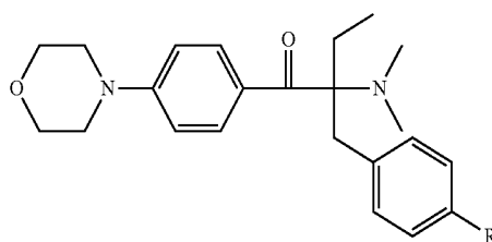
Chemical Formula 10
