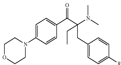
Chemical Formula 9
