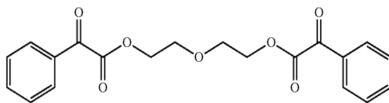
Chemical Formula 6
