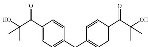
Chemical Formula 5
