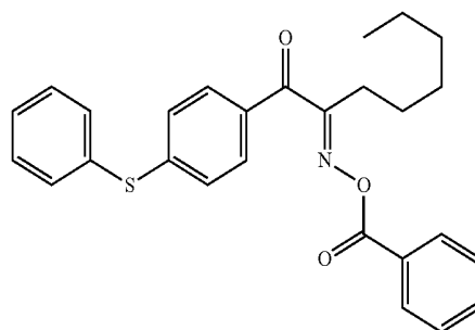
Chemical Formula 13
