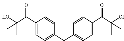
Chemical Formula 5
