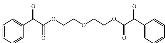
Chemical Formula 6
