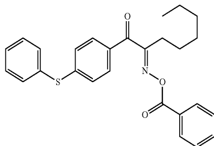
Chemical Formula 13
