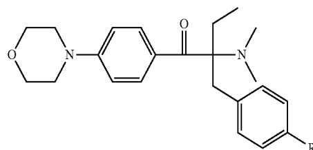
Chemical Formula 11
