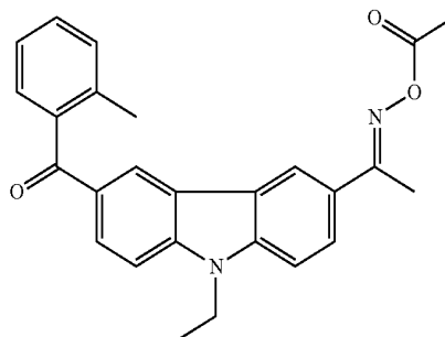
Chemical Formula 14
