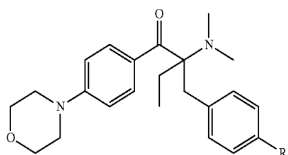
Chemical Formula 9
