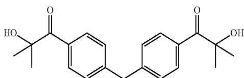
Chemical Formula 4
