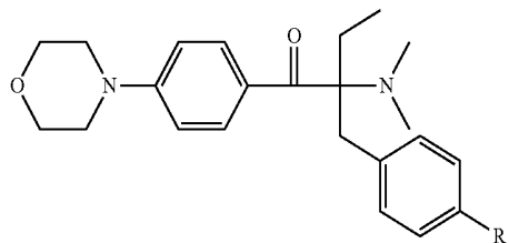
Chemical Formula 10
