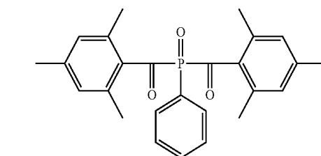
Chemical Formula 7
