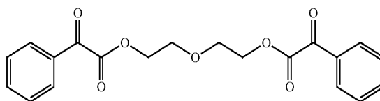
Chemical Formula 6
