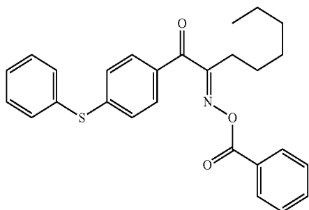
Chemical Formula 12
