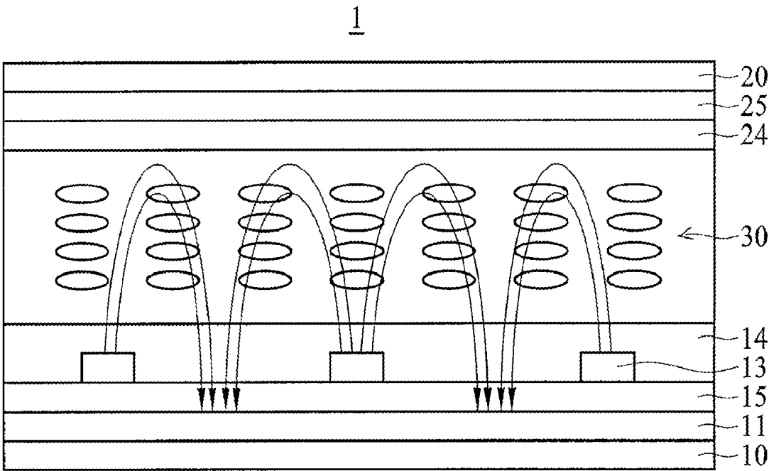
FIG. 1 (RELATED ART)
