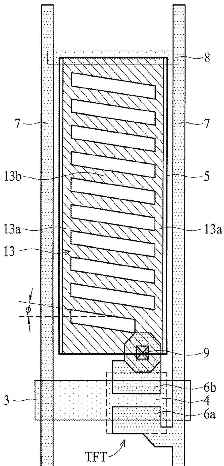
FIG. 2 (RELATED ART)
