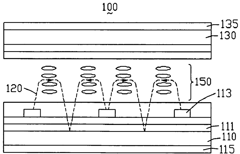
FIG. 10 (RELATED ART)
