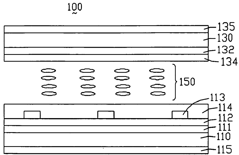
FIG. 9 (RELATED ART)
