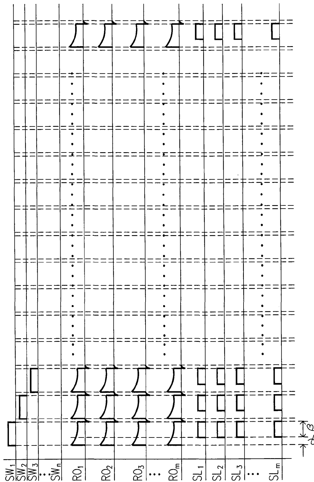
Fig. 5(PRIOR ART)
