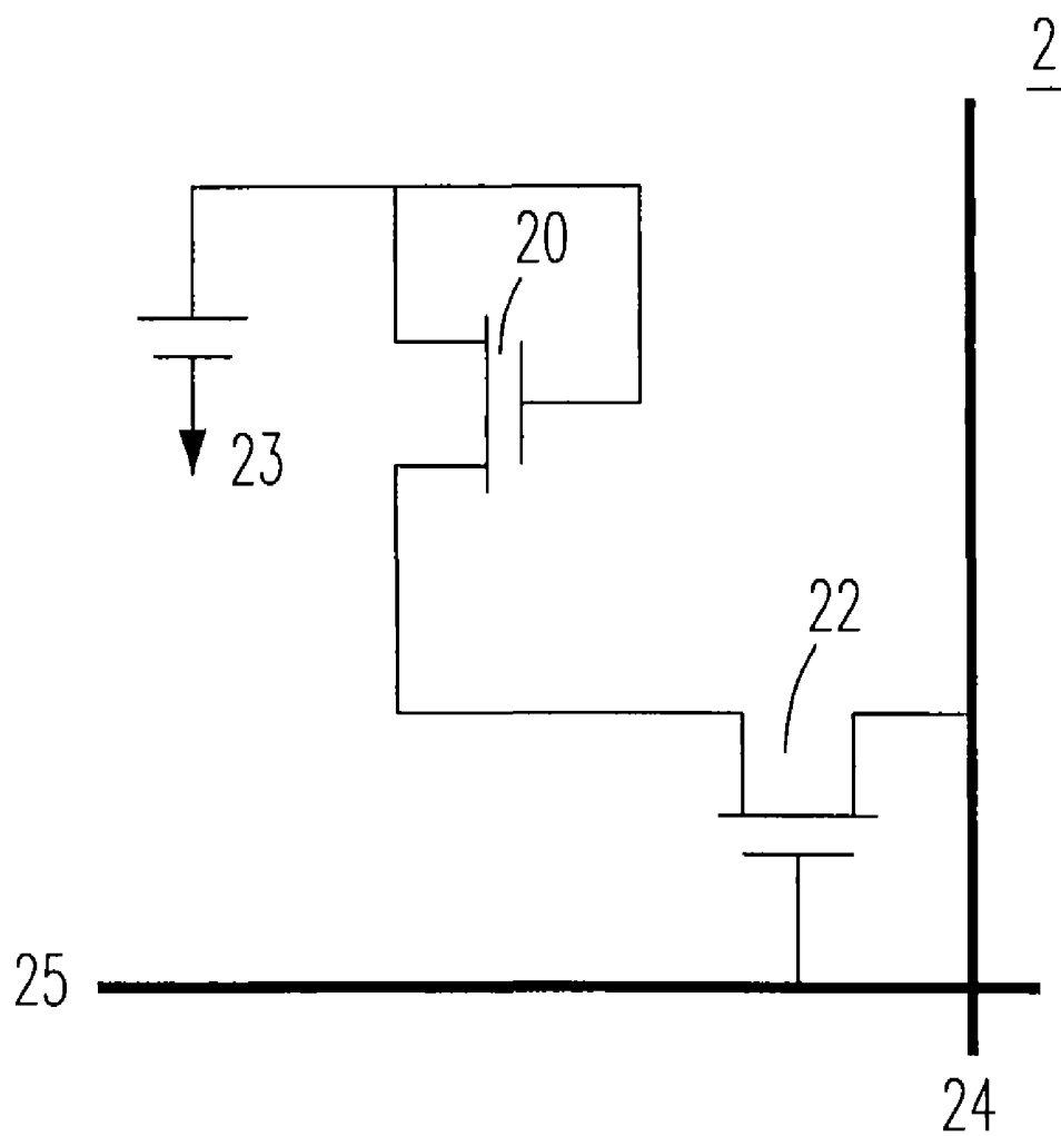
Fig. 2 (PRIOR ART)
