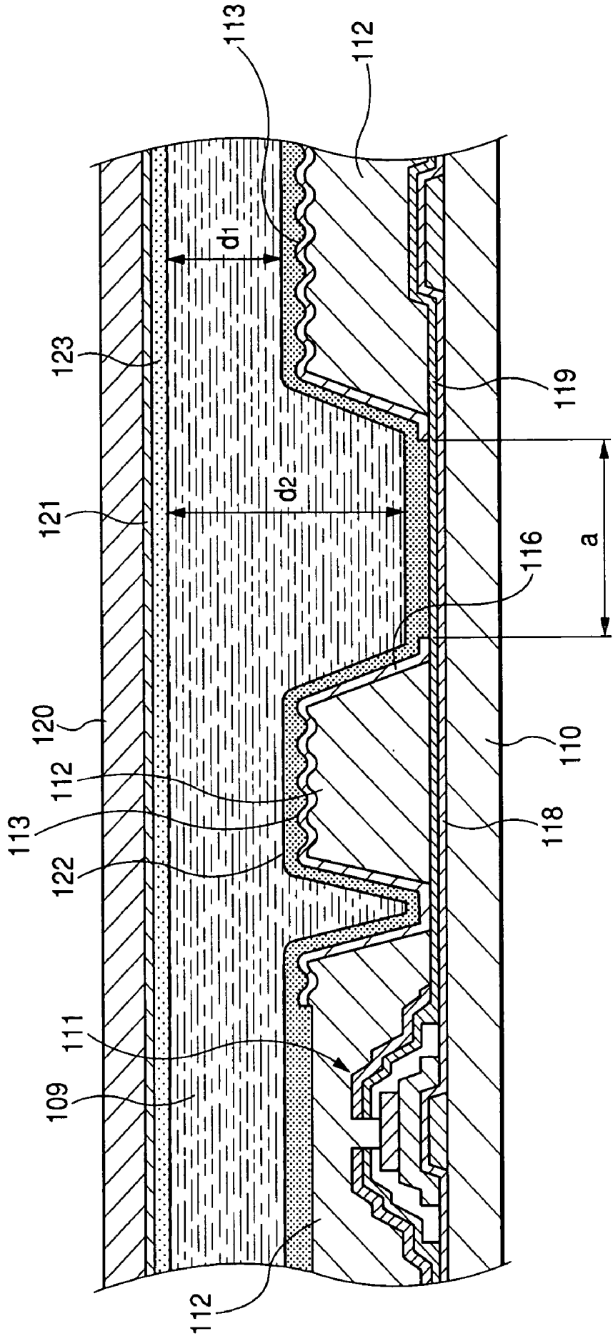
FIG. 13 PRIOR ART
