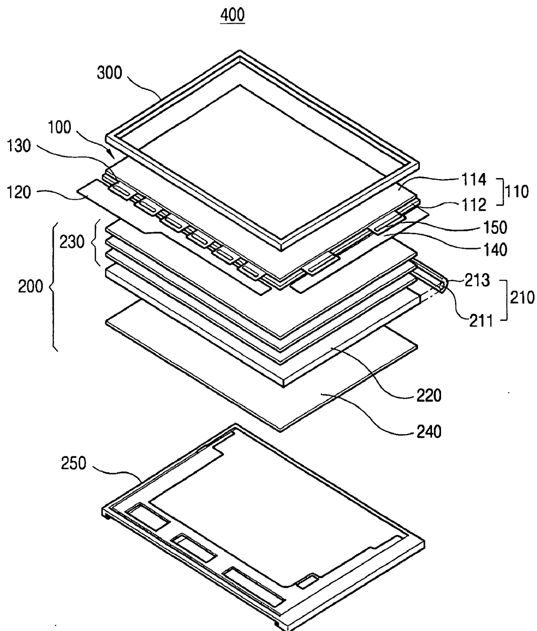
FIG. 1 (PRIOR ART)
