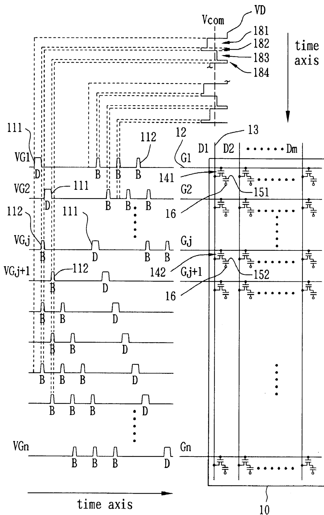
FIG. 1 (Background Art)
