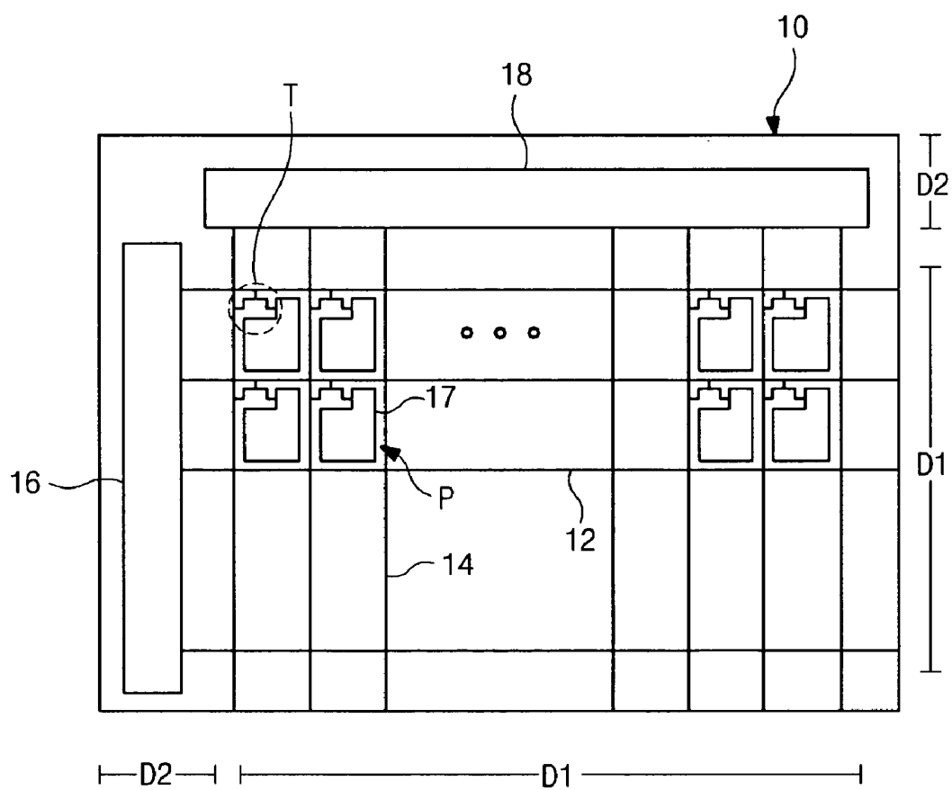
FIG. 1 RELATED ART
