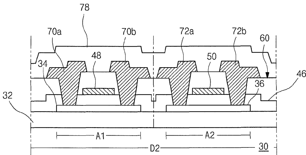
FIG. 4H PRIOR ART
