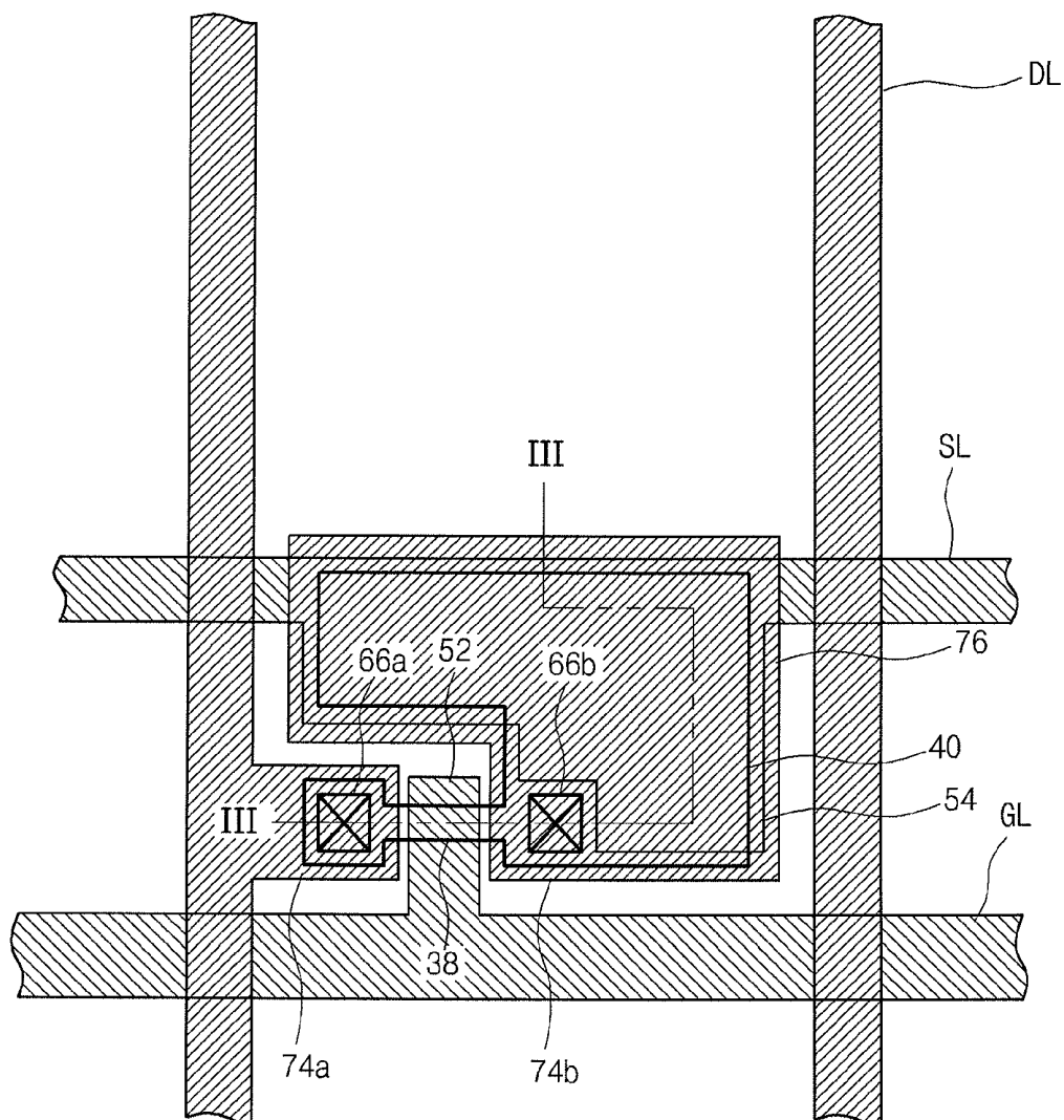
FIG. 5G PRIOR ART
