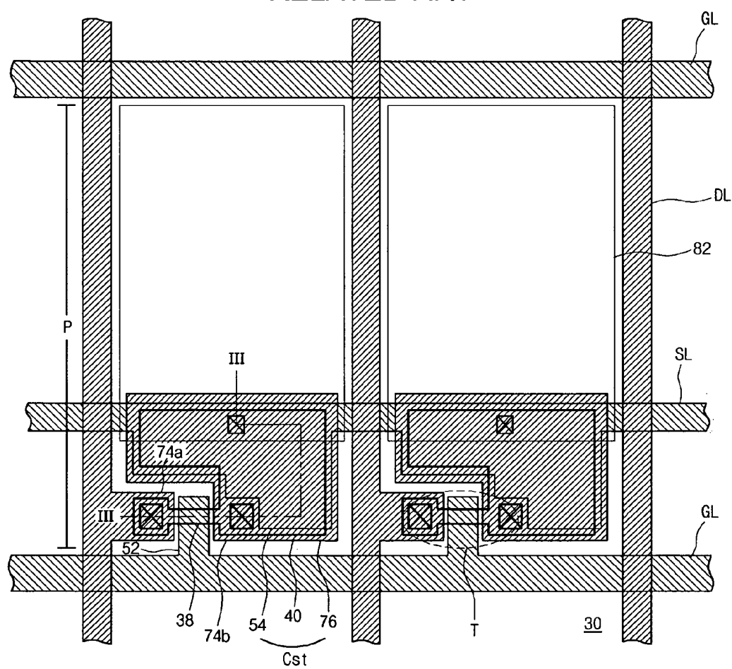
FIG. 2 RELATED ART
