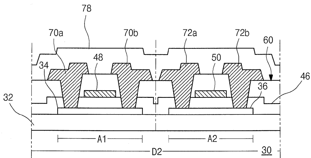
FIG. 4I PRIOR ART
