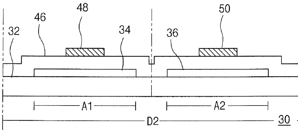
FIG. 4C PRIOR ART
