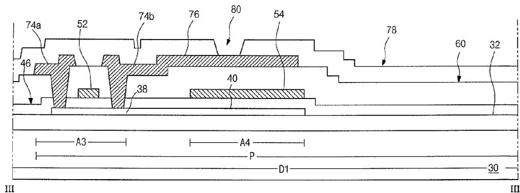
FIG. 6H PRIOR ART
