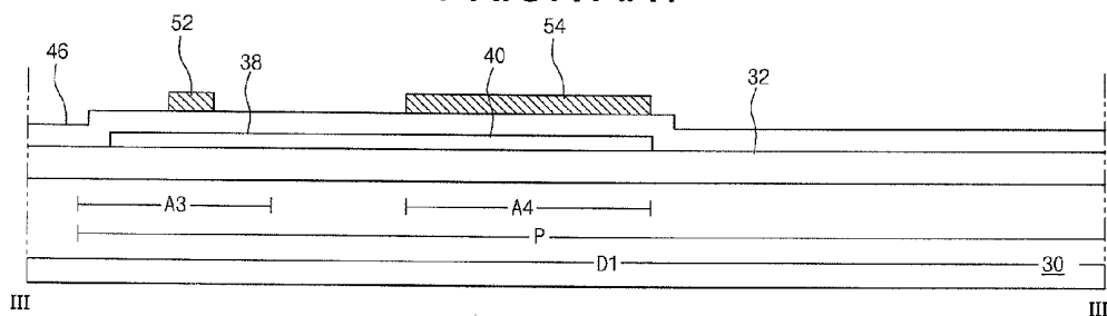
FIG. 6C PRIOR ART
