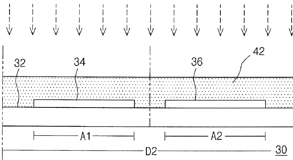
FIG. 4B PRIOR ART n + ion doping
