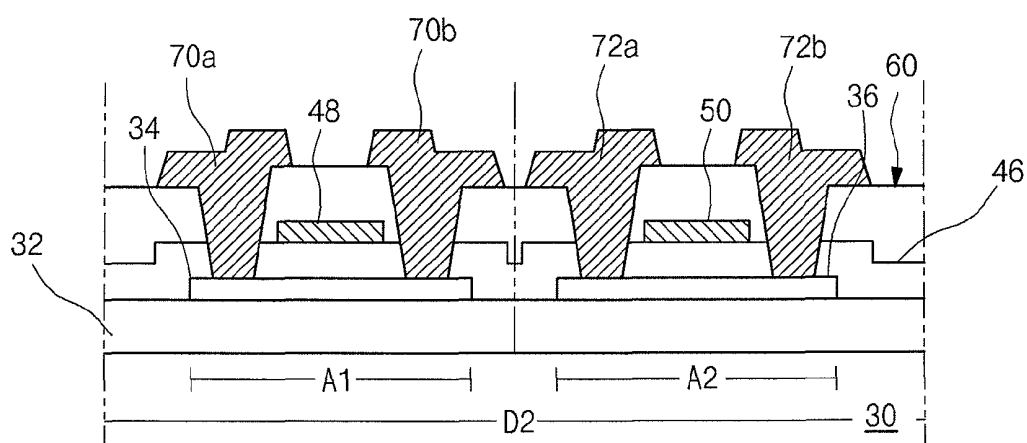
FIG. 4G PRIOR ART
