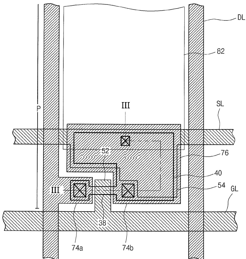
FIG. 5I PRIOR ART
