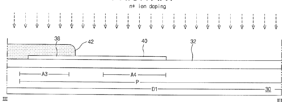
FIG. 6C PRIOR ART
