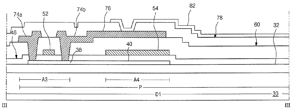
FIG. 6I PRIOR ART
