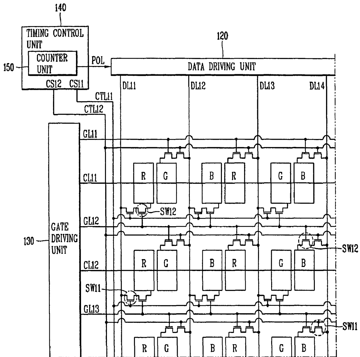
FIG. 3D
