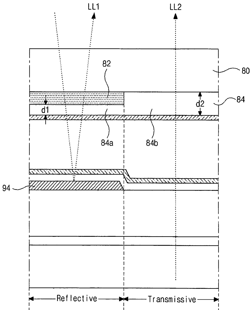
FIG. 2 RELATED ART
