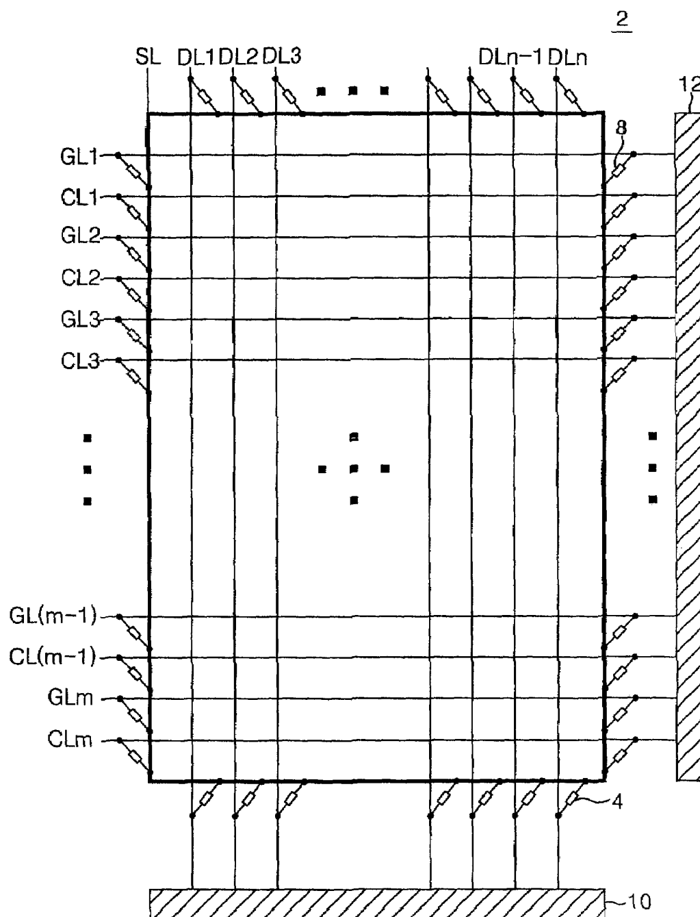
FIG.1 RELATED ART
