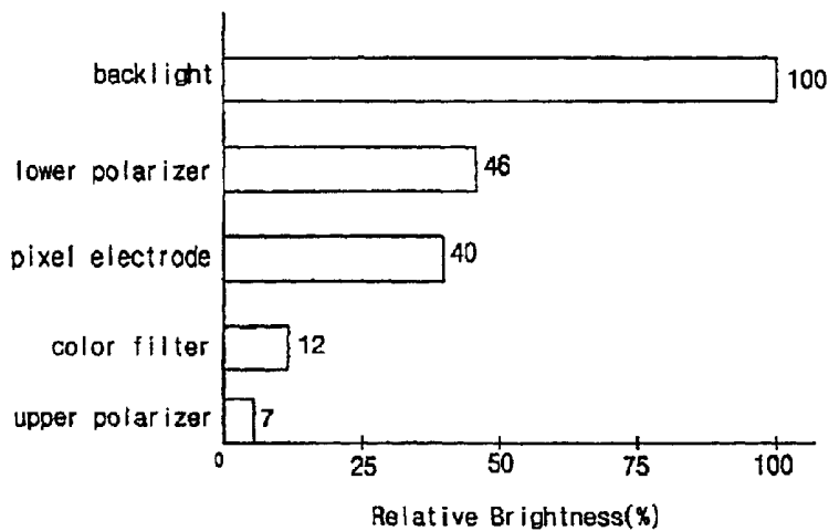
FIG. 3 (RELATED ART)
