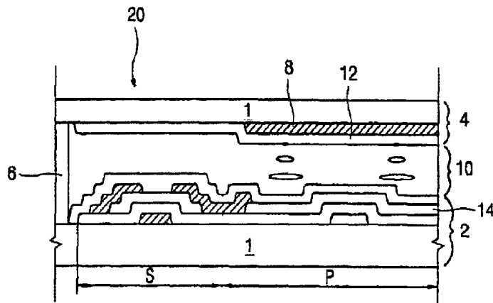
FIG. 1 (RELATED ART)
