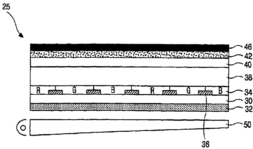
FIG. 2 (RELATED ART)
