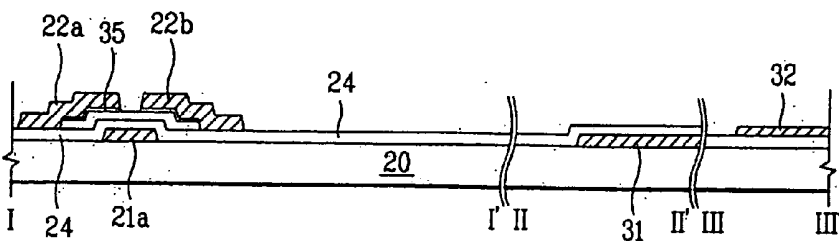
FIG. 4C Related Art
