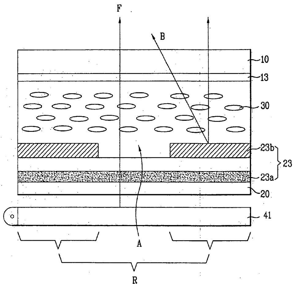
FIG. 2 Related Art
