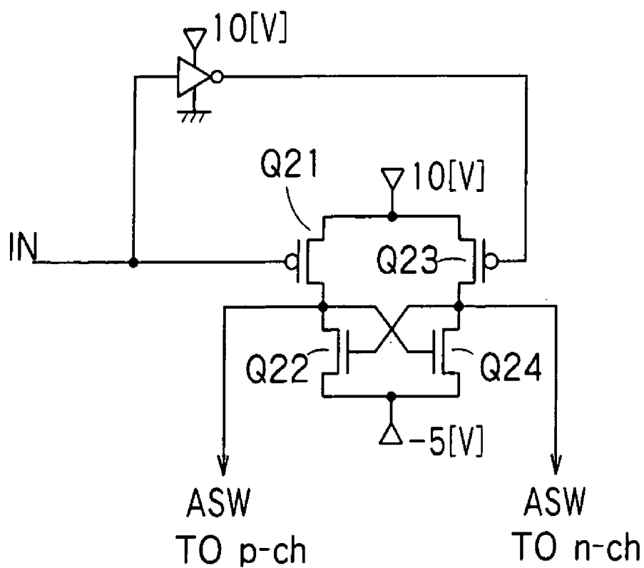
22: LEVEL CONVERSION CIRCUIT
