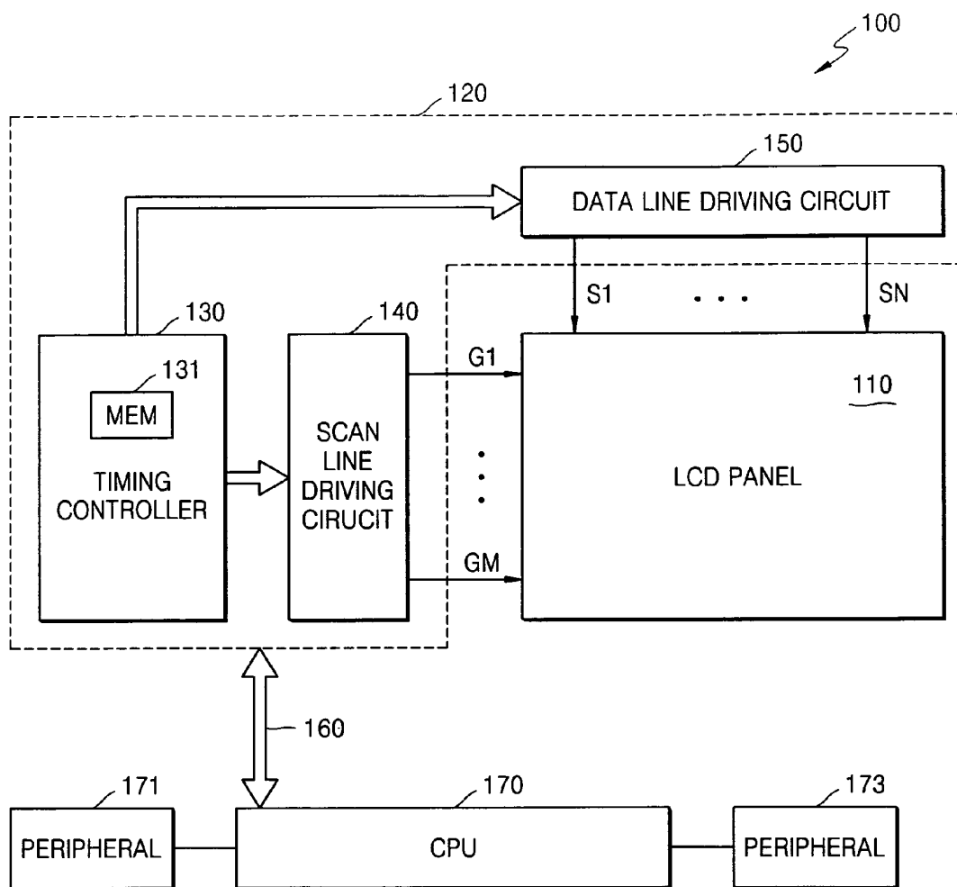
FIG. 1 (PRIOR ART)
