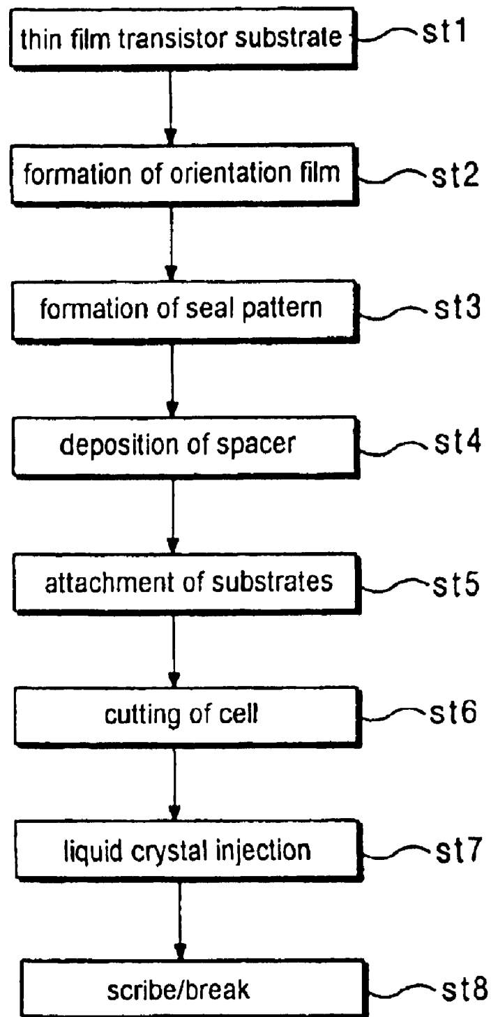
FIG. 2 (PRIOR ART)
