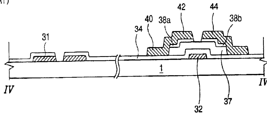
FIG. 4D (RELATED ART)
