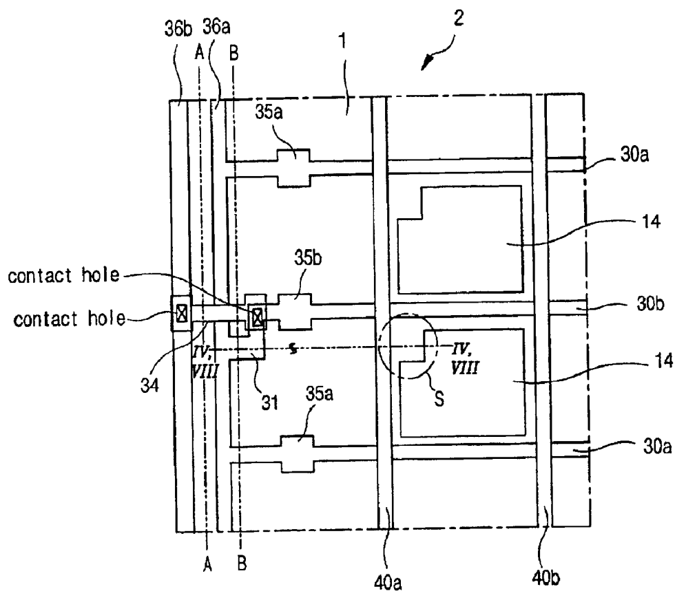
FIG. 4A (RELATED ART)
