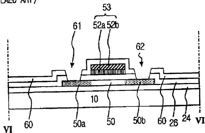
FIG. 6D (RELAED ART)
