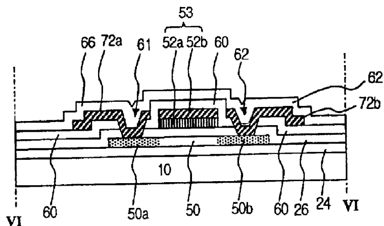
FIG. 6D (RELAED ART)
