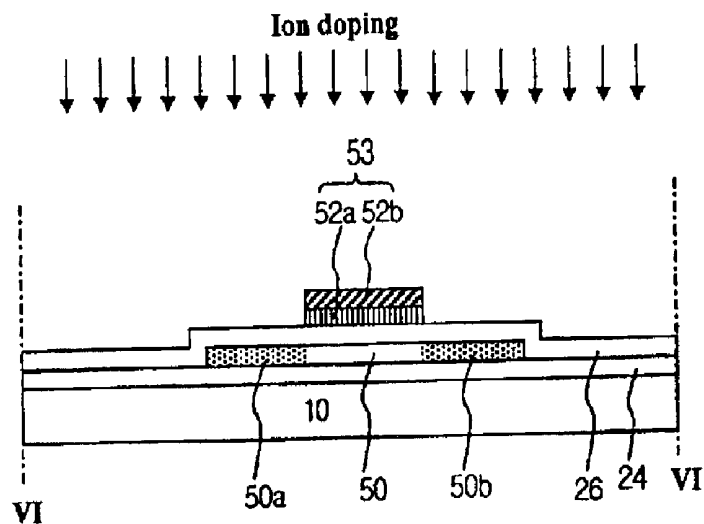
FIG. 6B (RELAED ART)
