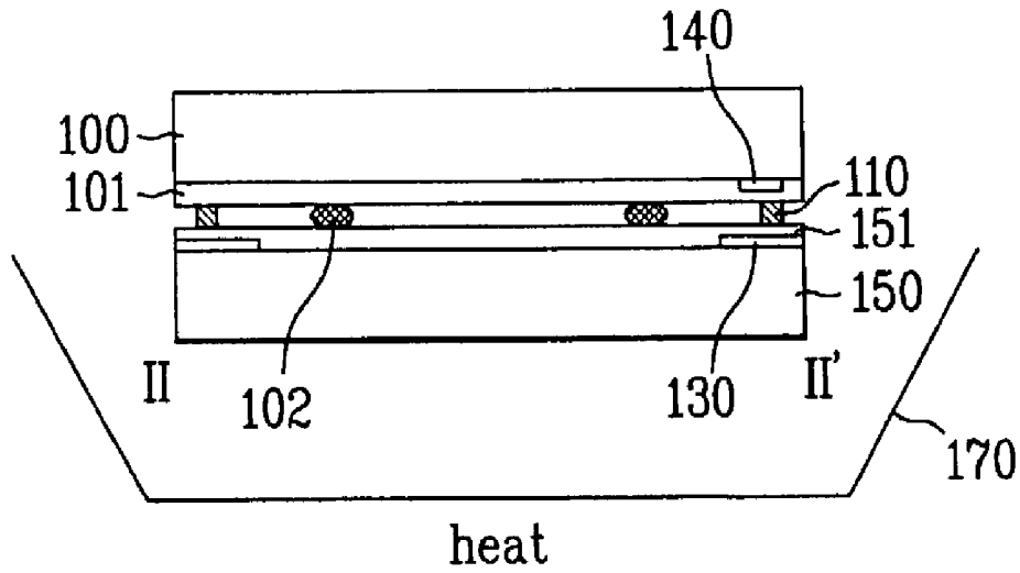
FIG. 4C Related Art
