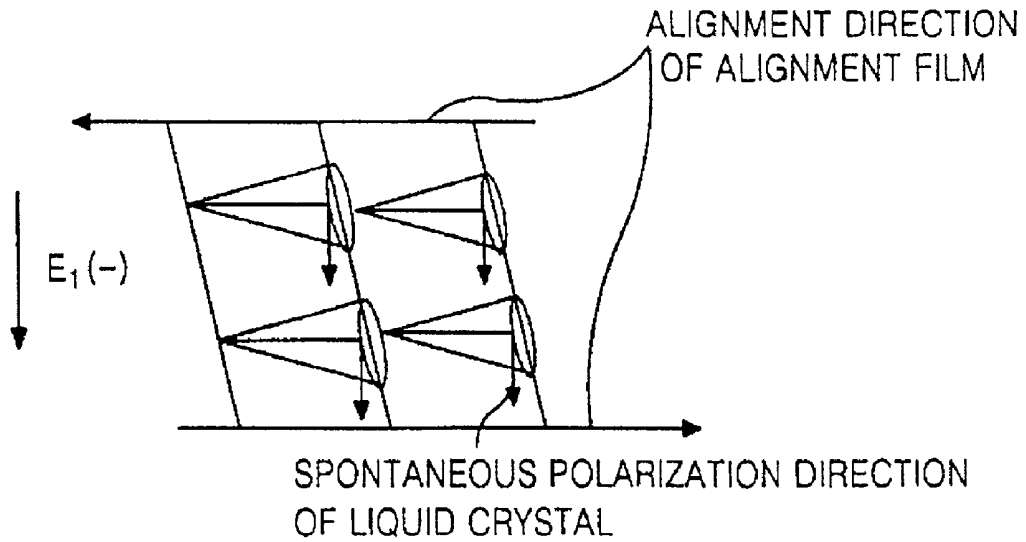
FIG. 5 CONVENTIONAL ART
