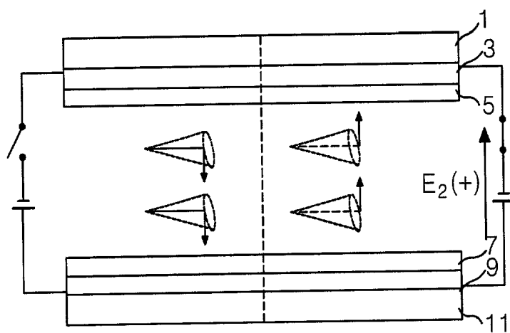
FIG. 6 CONVENTIONAL ART
