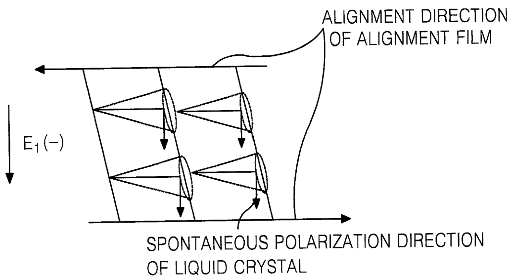
FIG. 5 CONVENTIONAL ART
