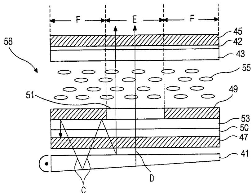
Fig.3 (Related Art)
