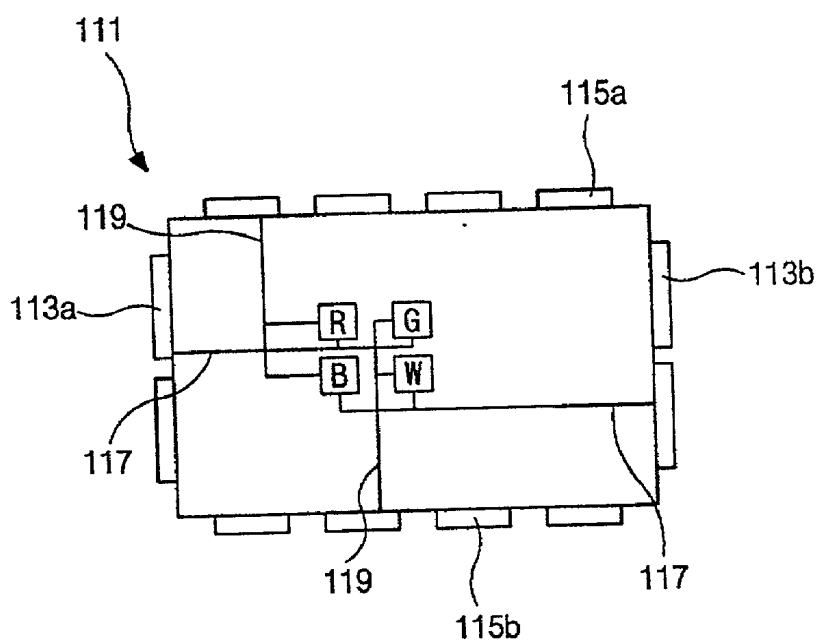
FIG.3 (RELATED ART)
