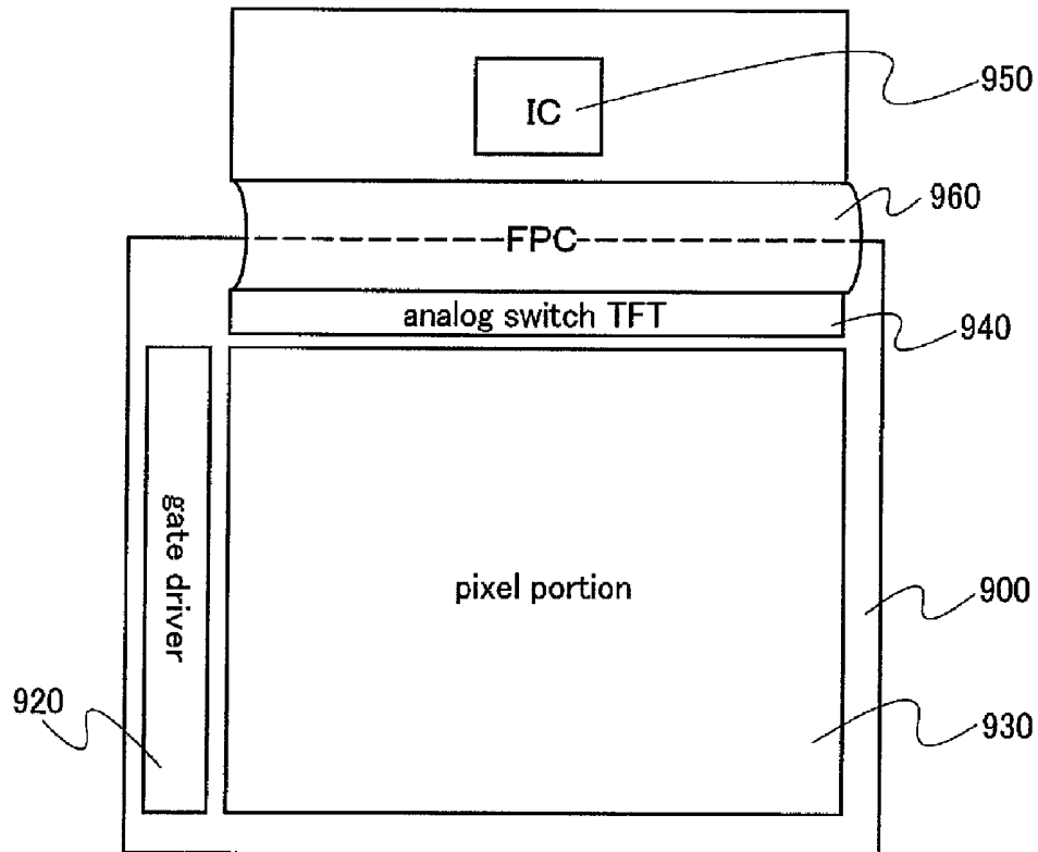
FIG. 17A IC connected by FPC
