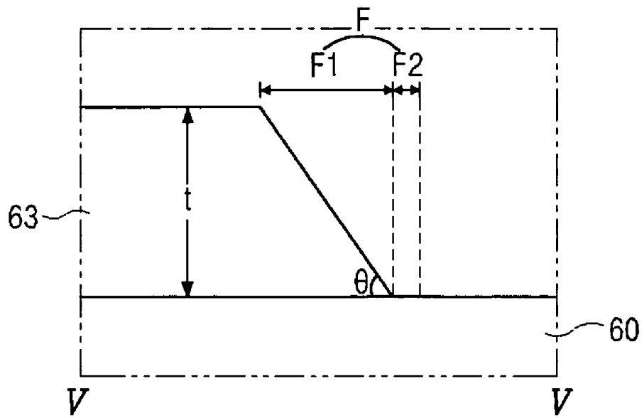
FIG. 5 RELATED ART
