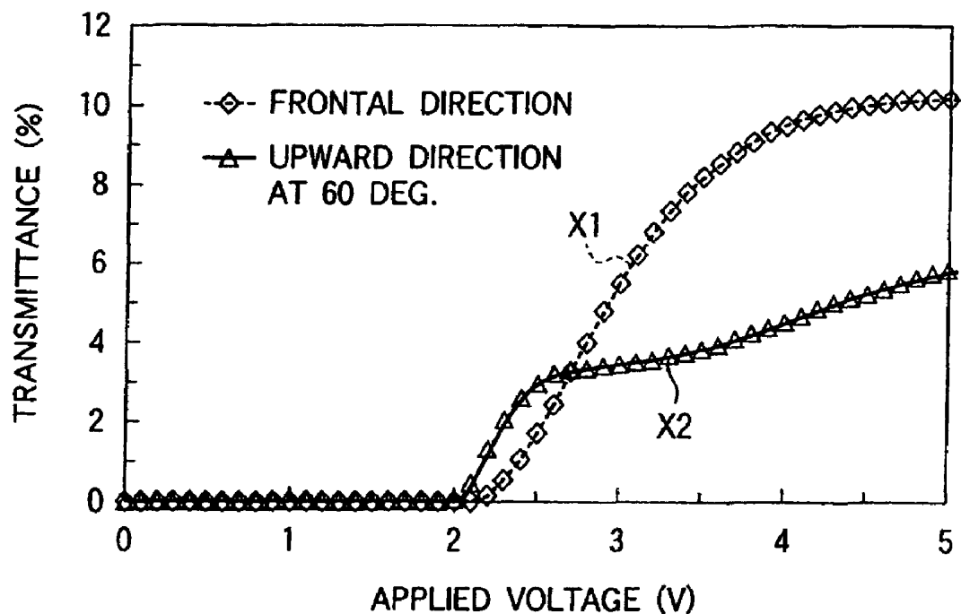
FIG.18 PRIOR ART
