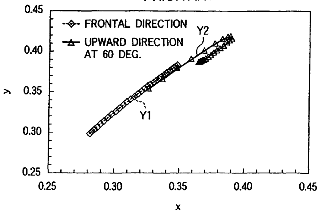
FIG.19 PRIOR ART
