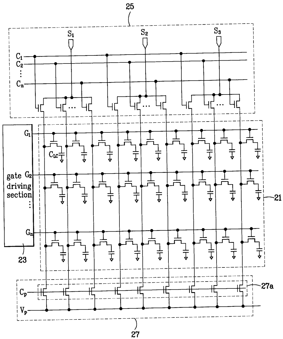
FIG. 2 Related Art
