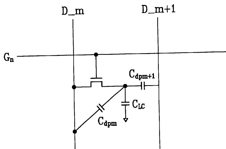
FIG. 4 Related Art
