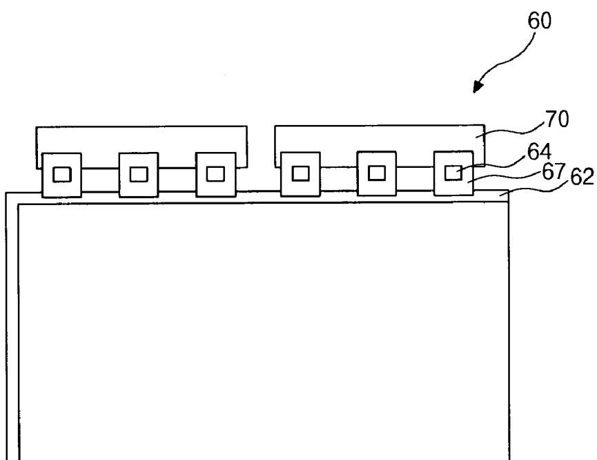
FIG. 4 RELATED ART
