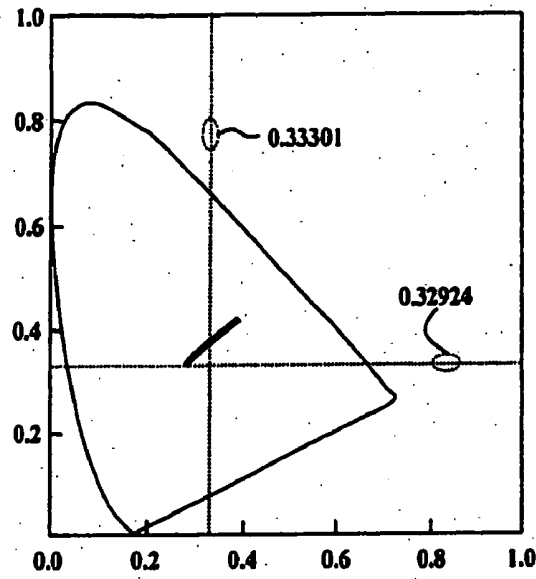
FIG. 6 (RELATED ART)
