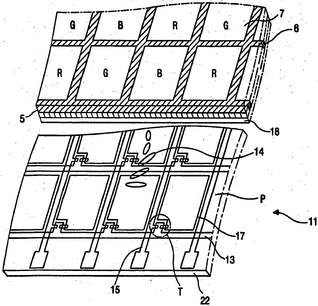
FIG. 1 (RELATED ART)
