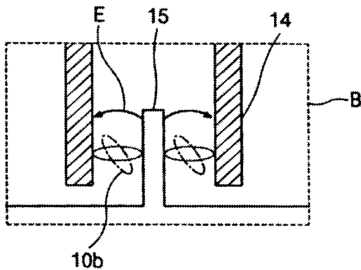
(prior art) FIG. 9B
