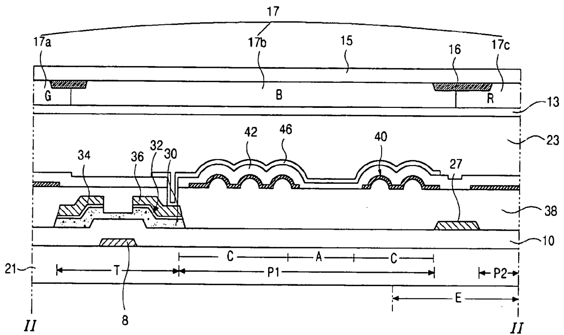
FIG. 2 RELATED ART
