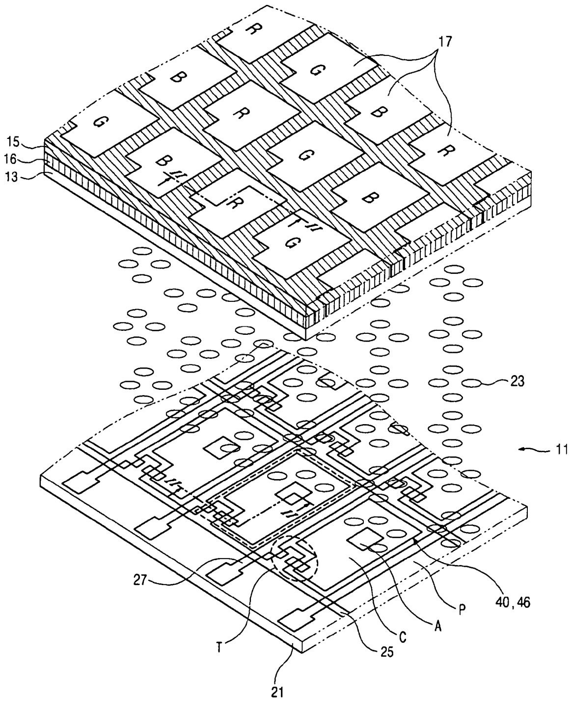
FIG. 1 RELATED ART
