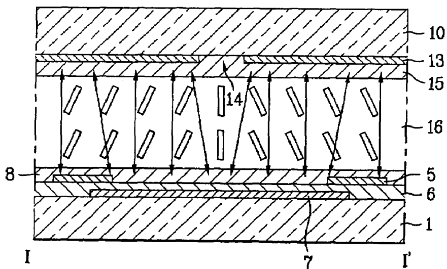
FIG.2 Related Art
