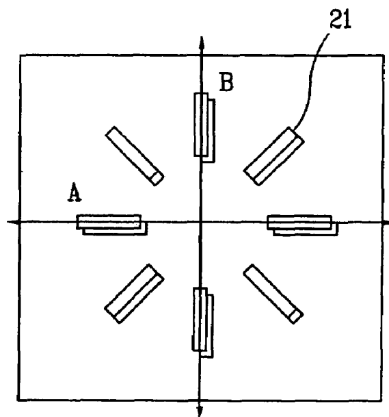
FIG. 3 Related Art
