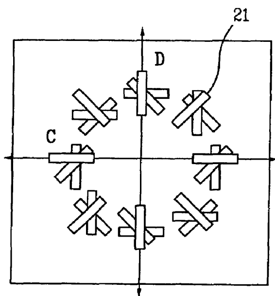
FIG. 4 Related Art
