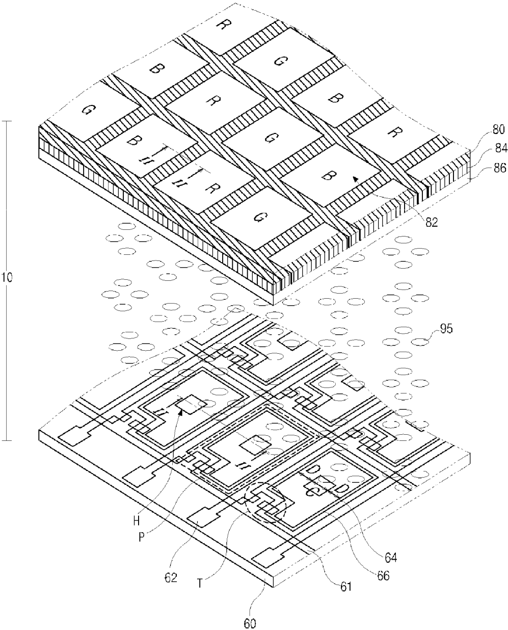
FIG. 1 RELATED ART
