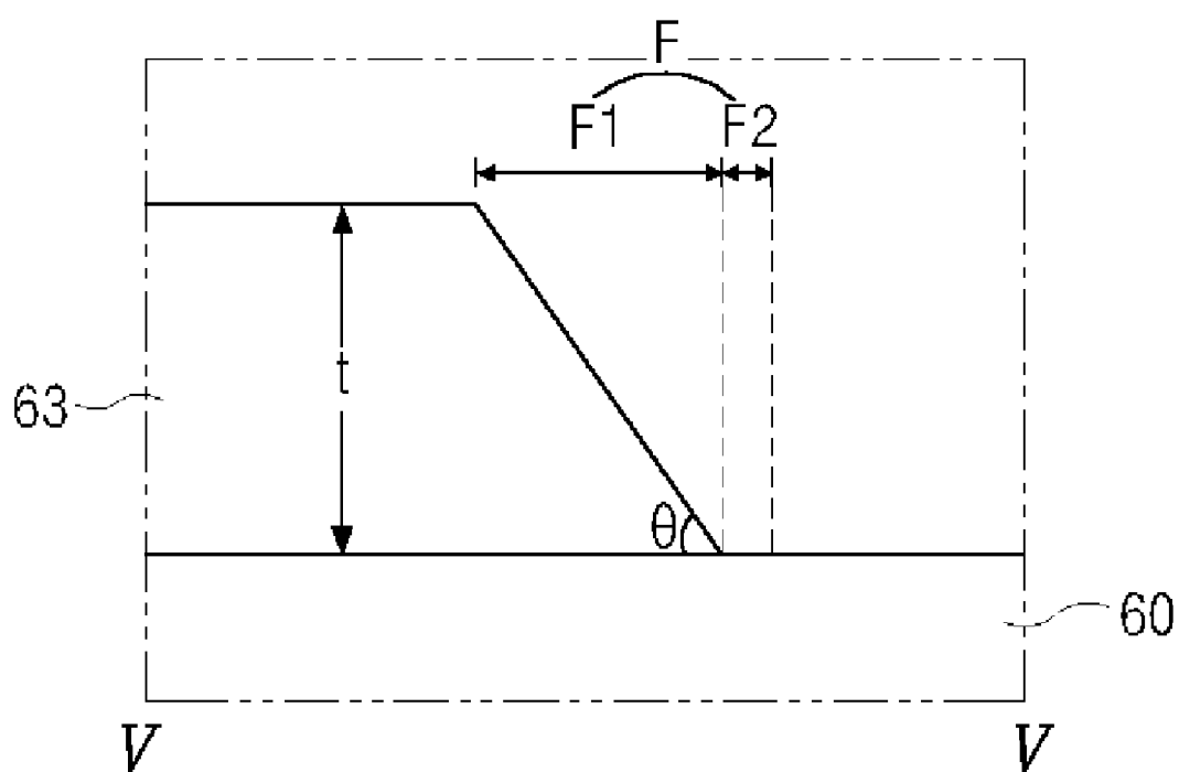
FIG. 5 RELATED ART
