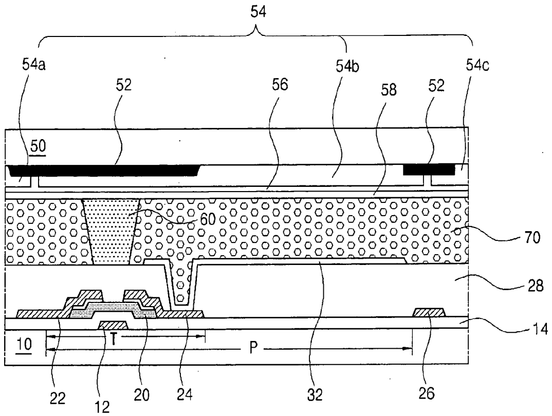
FIG. 3 RELATED ART
