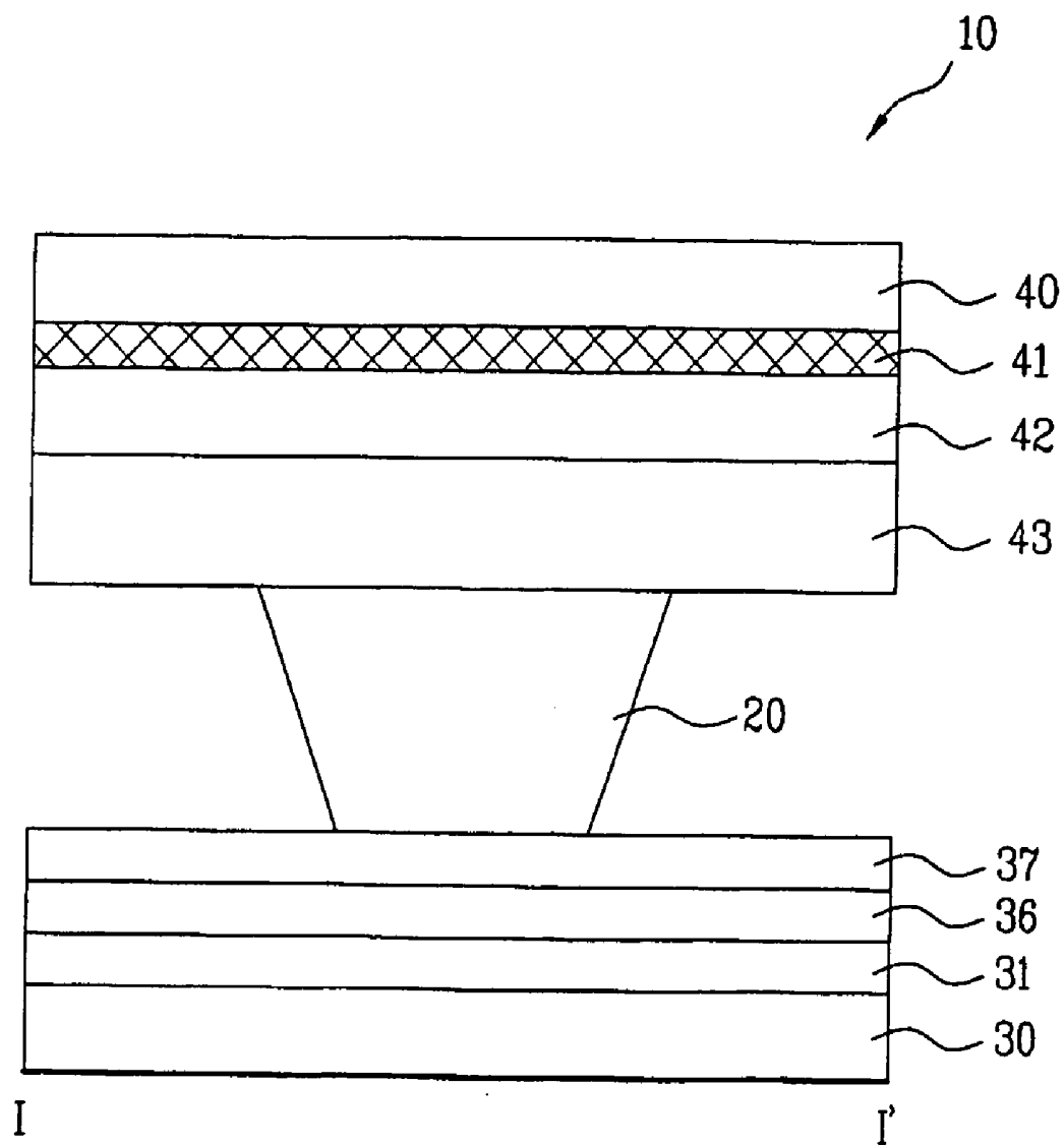
FIG. 2 Related Art
