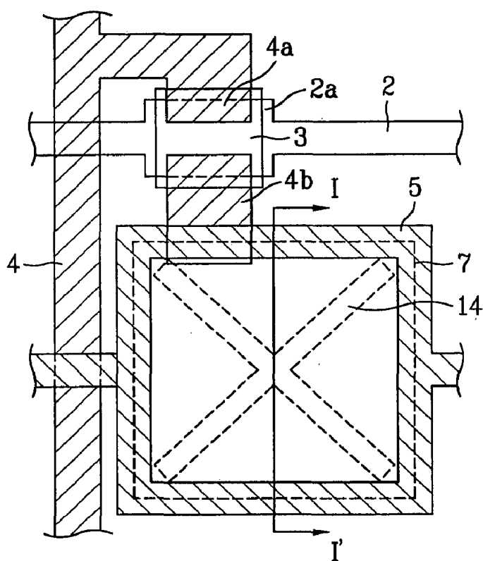
FIG.2 Related Art
