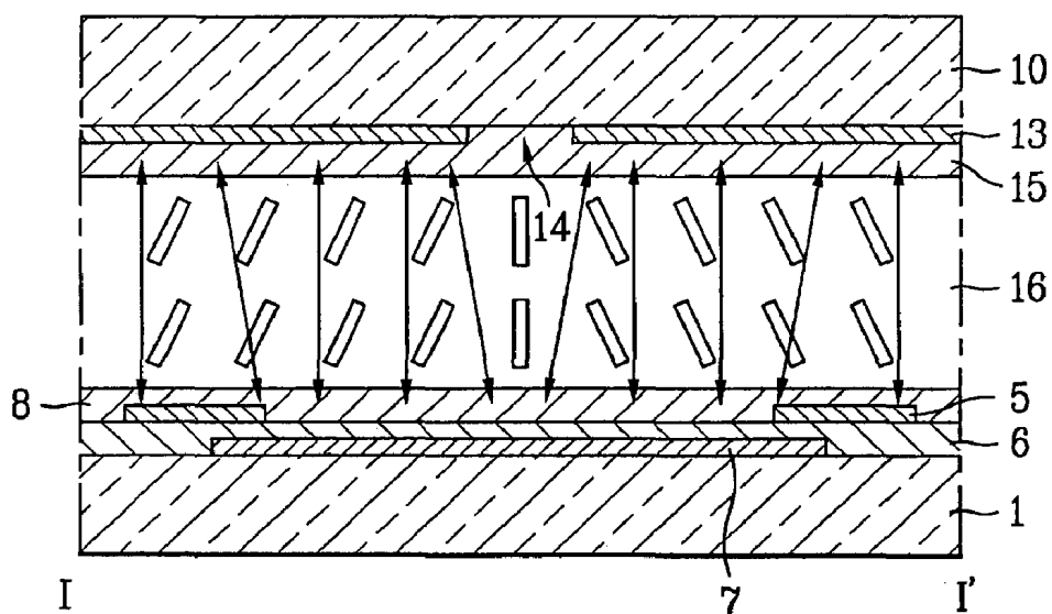
FIG.2 Related Art
