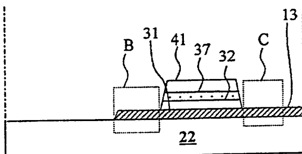
FIG.9 (RELATED ART)
