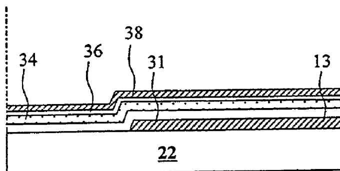
FIG.5 (RELATED ART)
