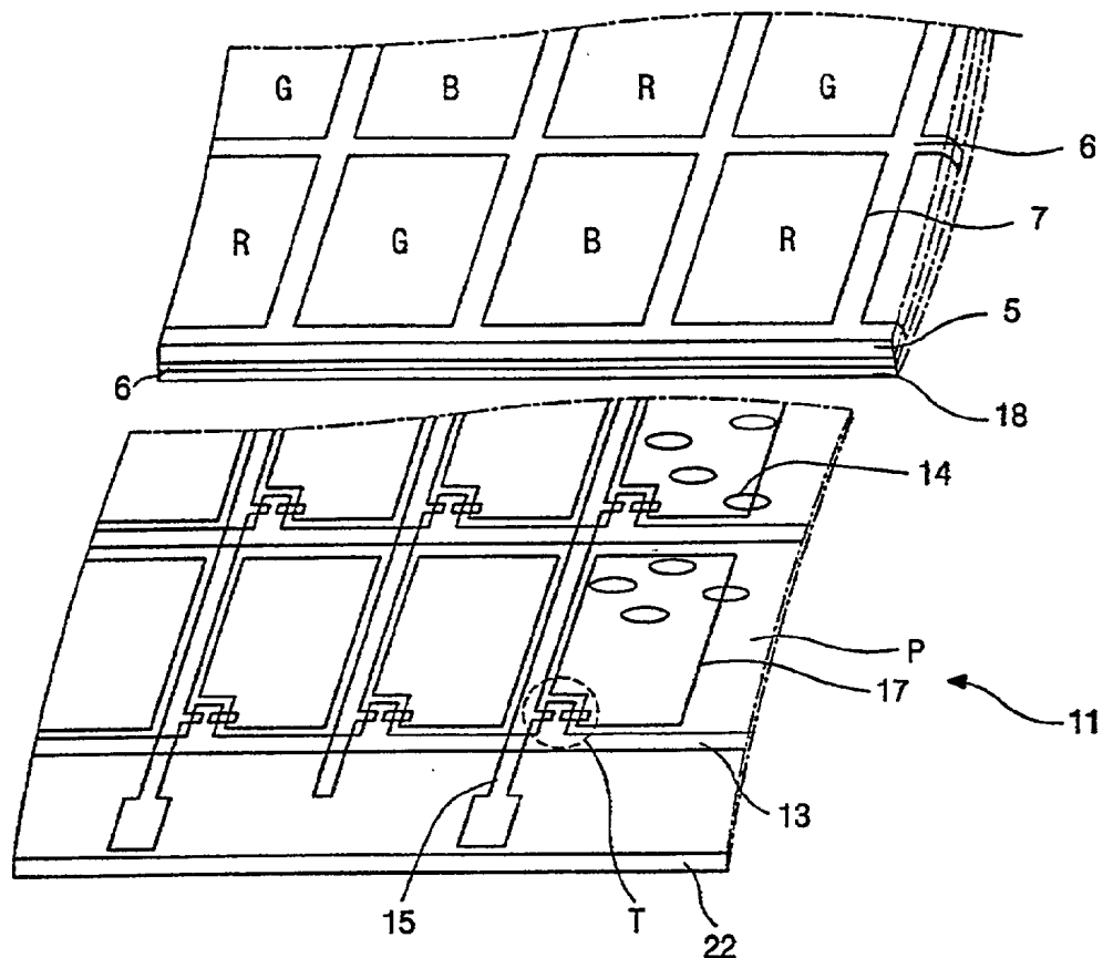
FIG.1 (RELATED ART)
