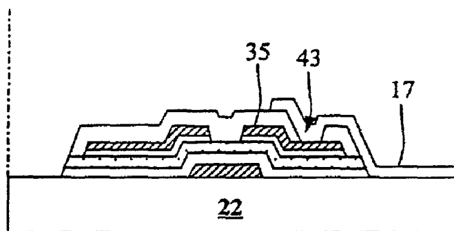
FIG.10 (RELATED ART)
