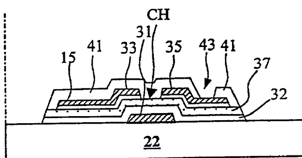
FIG.8 (RELATED ART)
