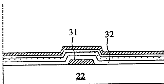
FIG.4 (RELATED ART)
