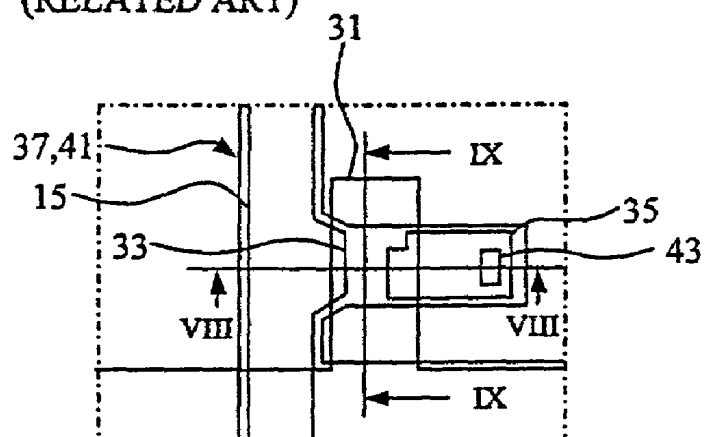
FIG.3C (RELATED ART)
