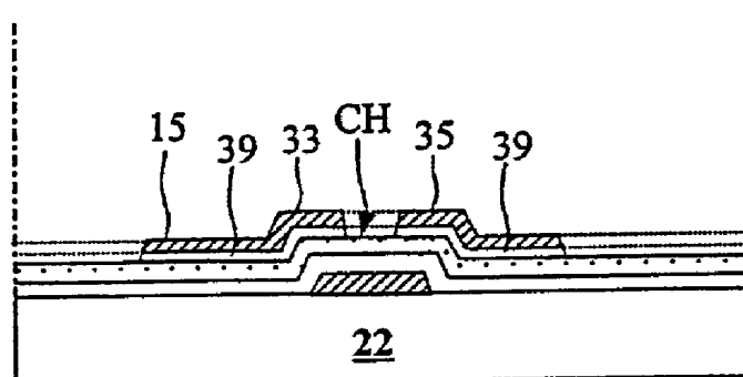
FIG.6 (RELATED ART)
