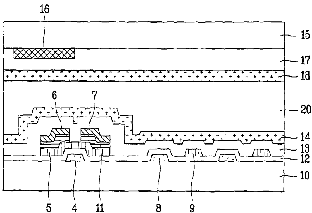
FIG. 2 Related Art
