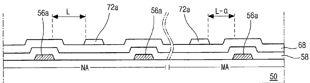
FIG. 4 Related Art
