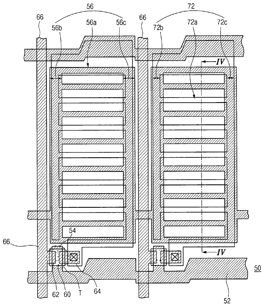
FIG. 3 Related Art
