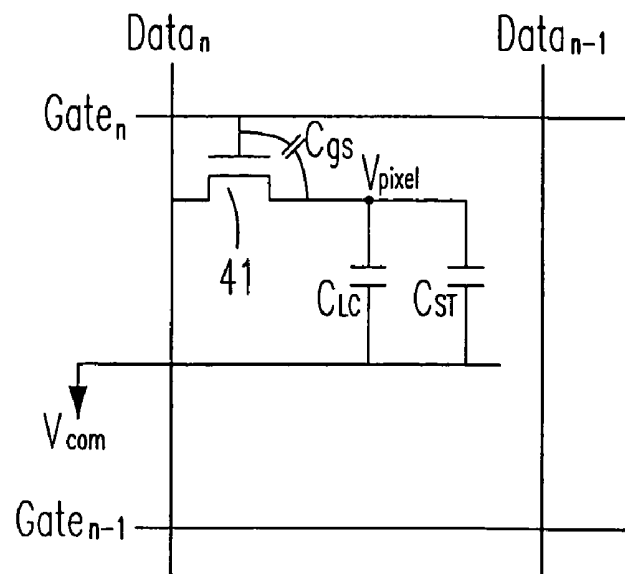
Fig. 4(a)(PRIOR ART)
