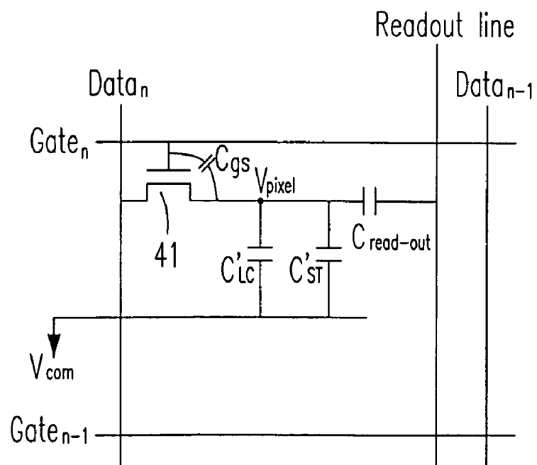
Fig. 4(b)(PRIOR ART)
