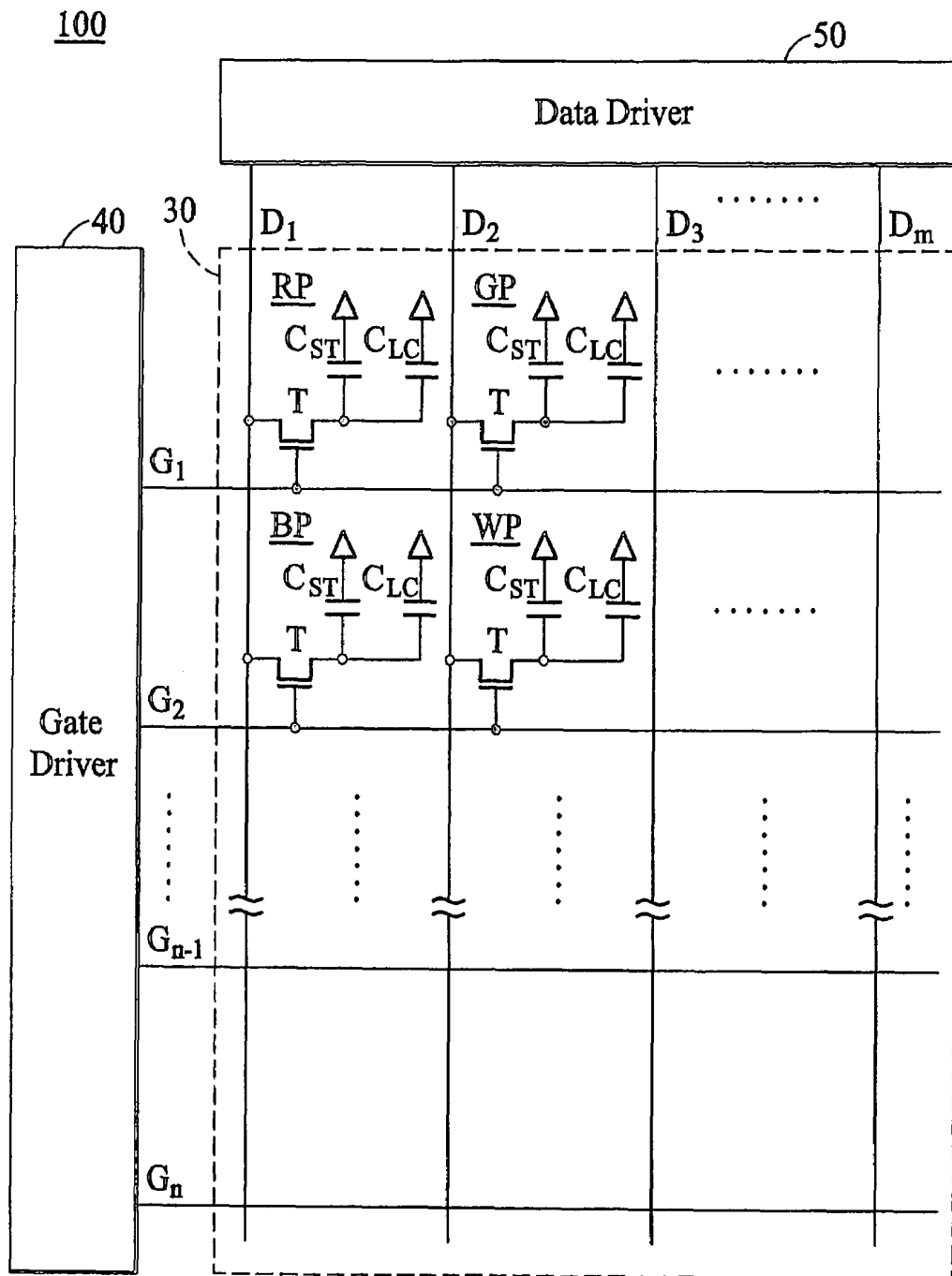
FIG. 2 (RELATED ART)
