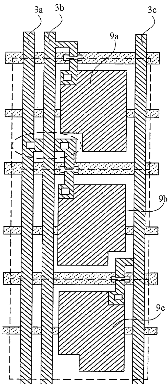
FIG. 5 (Prior art)
