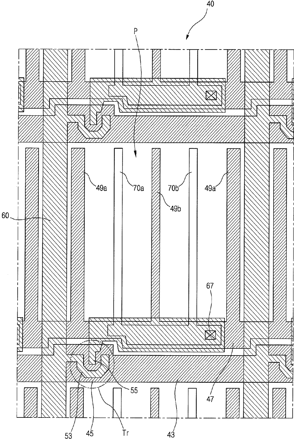
FIG. 3 RELATED ART
