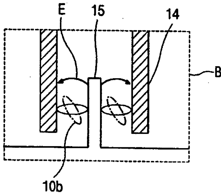
(related art) FIG. 9B
