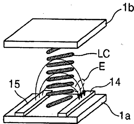
(related art) FIG 4B
