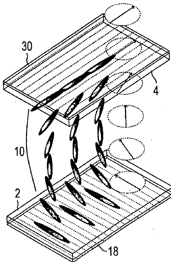
(related art) FIG. 2A
