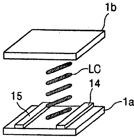
(related art) FIG 4A
