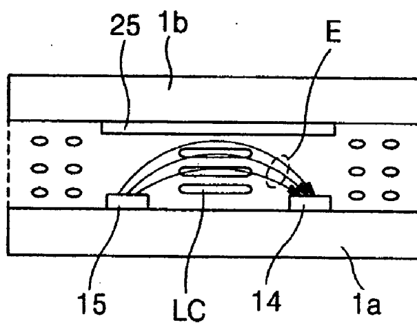
(related art) FIG. 3
